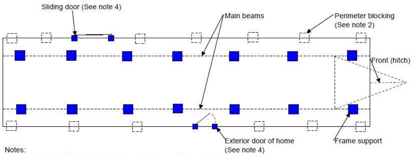
FIGURE 6.2.5.3 Typical Blocking Diagram for a Single Section
