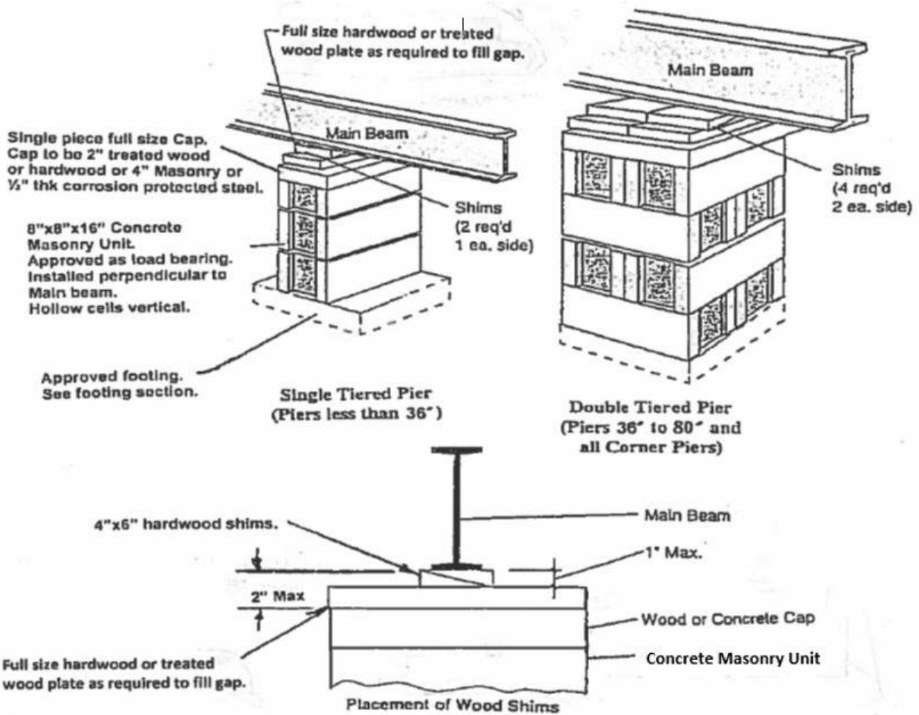
FIGURE 2.3 –Concrete Block Pier Construction
