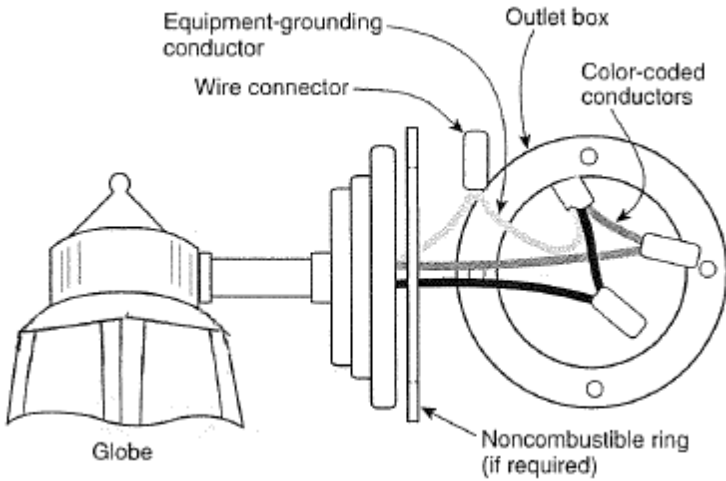
Figure 6.4-Exterior lighting fixtures
