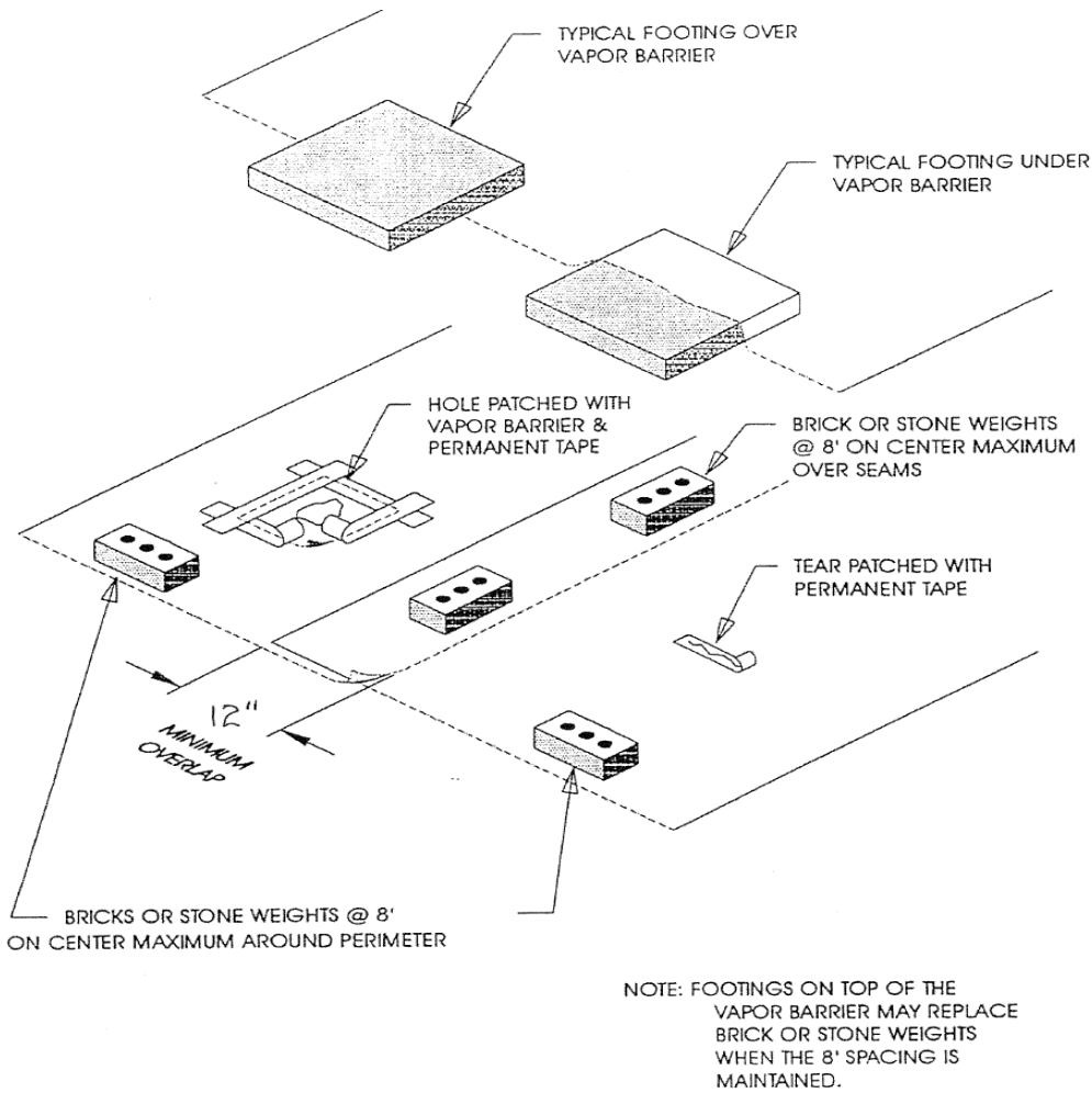
FIGURE 2.2 – Vapor Retarder Installation
