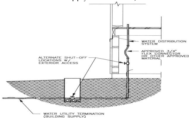
FIGURE 5.1 – Water Connection to Home
