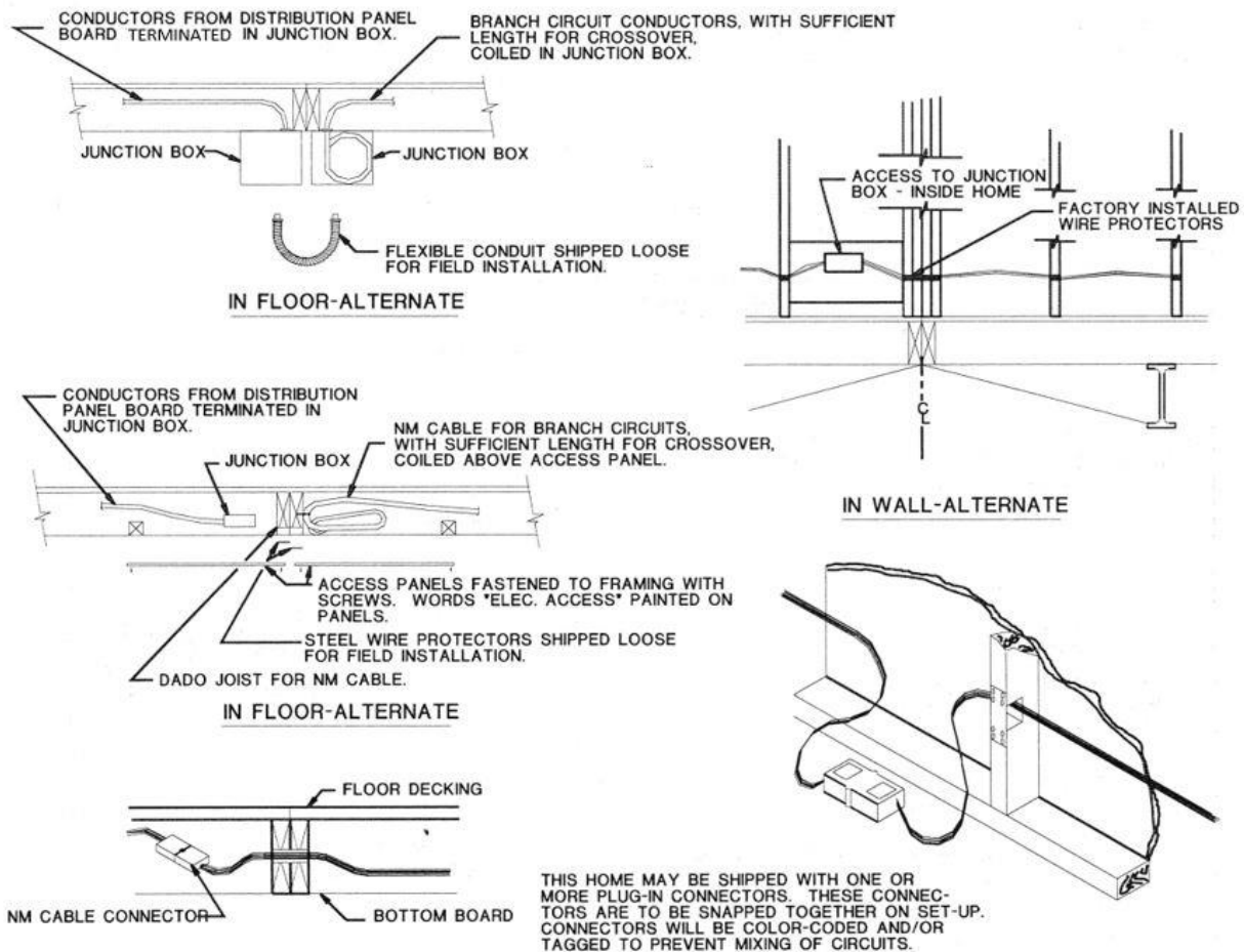
Figure 6.3 – Electrical Crossovers
