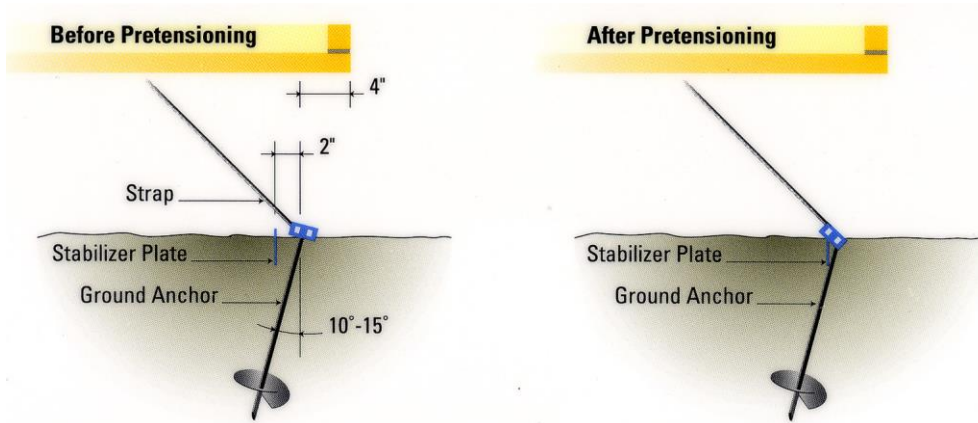
FIGURE 2.12 – Anchor Installation
