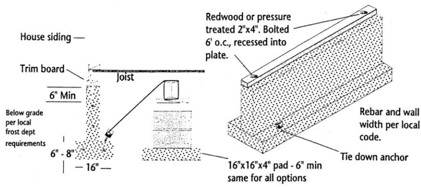
FIGURE 2.14 – Poured Concrete Foundation
