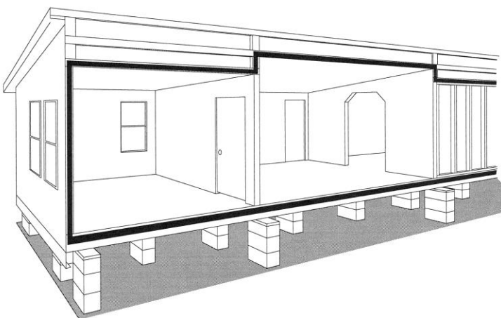
FIGURE 4.1 – Mating Line Insulation
