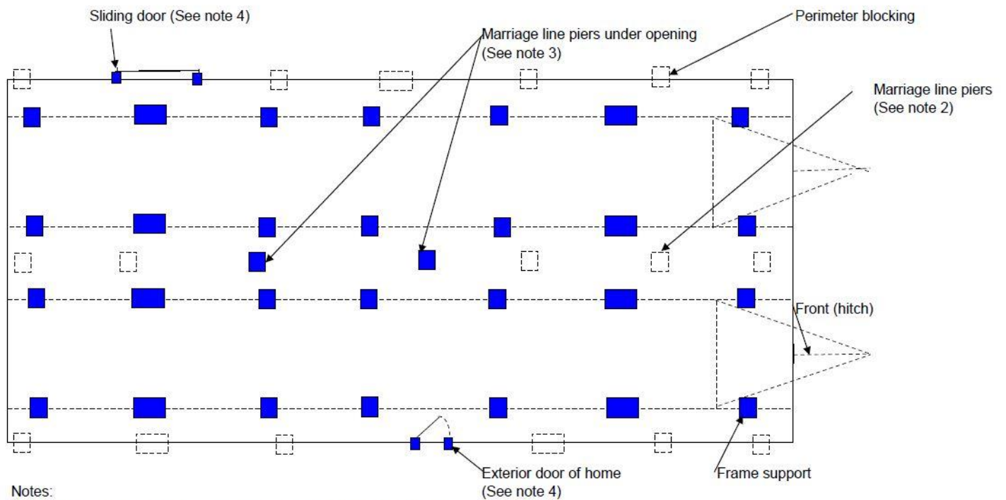
FIGURE 6.2.5.4 Typical Blocking Diagram for a Multi-Section Home
